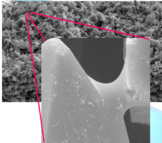
The perfect vitrified bonding bridge for ultra fine diamond grits
